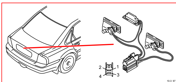
10/3 牌照燈
