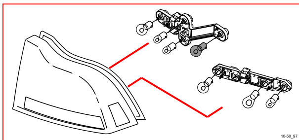
10/50 左煞車燈
