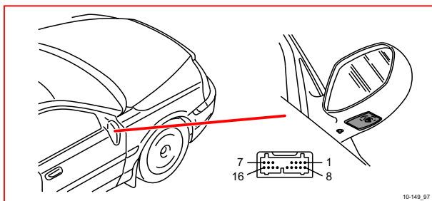
10/149 右側後視鏡照明燈
